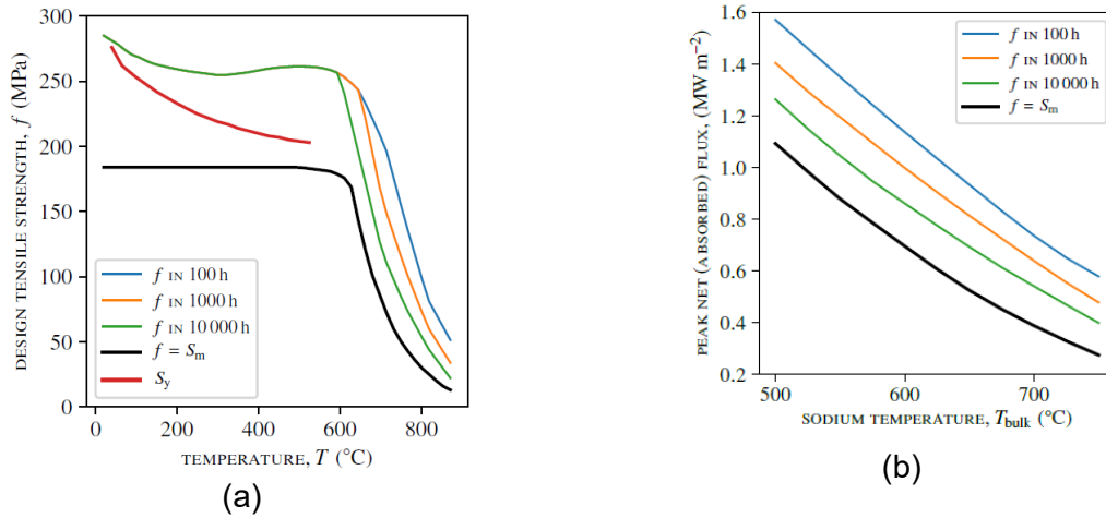
Figure 3. (a) Design tensile stress f for Alloy 625 showing time-dependent values derived from manufacturer's data compared to time-independent ( S_m ) allowable stress values from ASME BPVC II, Part D. (b) Peak allowable net flux (that which is absorbed by the tube, not including loss to ambient via radiation and convection) for UNS N06625 using creep-rupture data from manufacturer's data-sheets and ASME allowables for a mass flow of 0.18 \text{ kg s}^{-1} .
