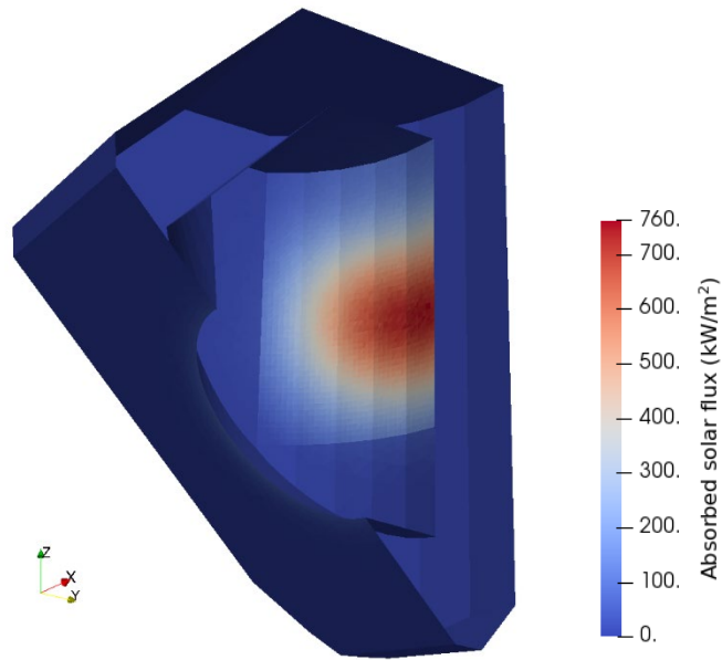
Figure 1. Heliosim 3D surface model of the conceptual receiver design, with a section mid receiver showing the predicted absorbed solar flux at design point.
