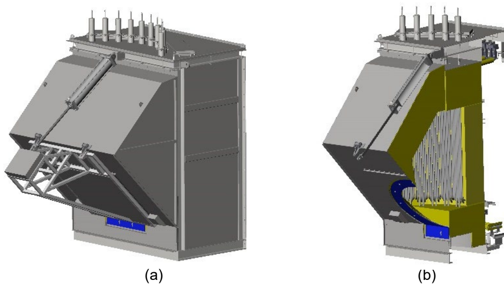
Figure 6. 3D models of the sodium receiver showing (a) the full receiver, including the door in the closed position, and (b) a section view through the centre of the receiver, with the door removed to show the aperture.
