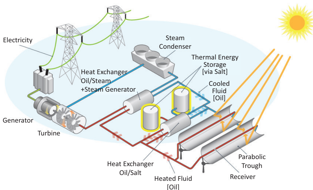
Figure 1: Working principle of CSP
