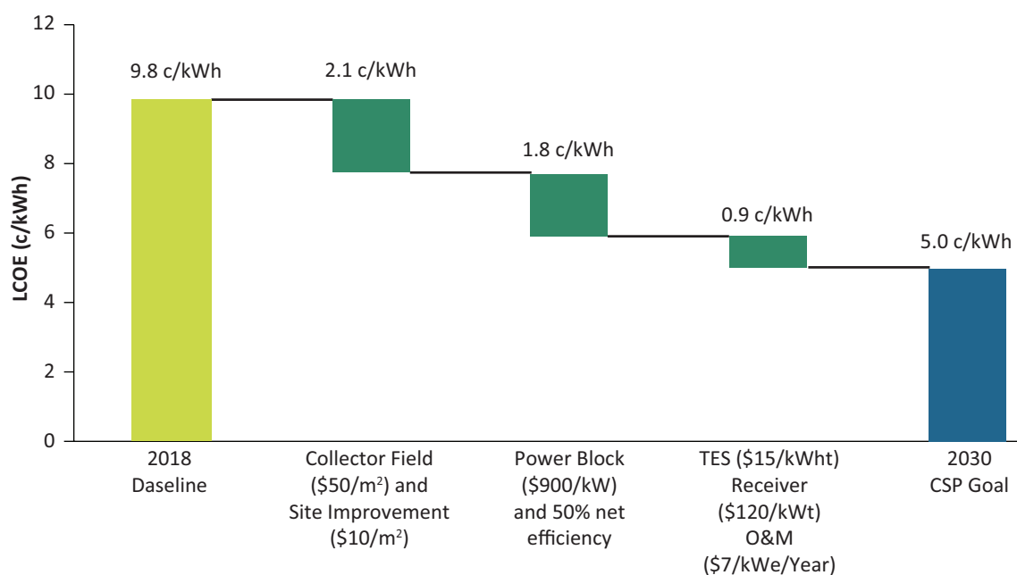
Figure 19: Performance and cost improvements contribute to reach the 2030 target for CSP LCOE
