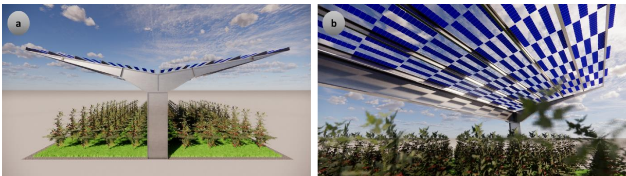
Figure 6: The overall view (a) and bottom view (b) of the Agri voltaic system pre-design.
