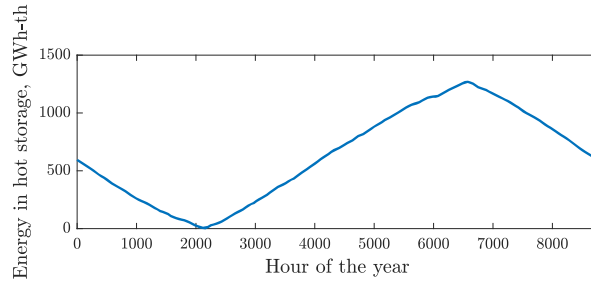
Figure 8: Energy capacity of the GeoTES during one year of operation. The GeoTES is depleted in winter months and recharged in summer months.
