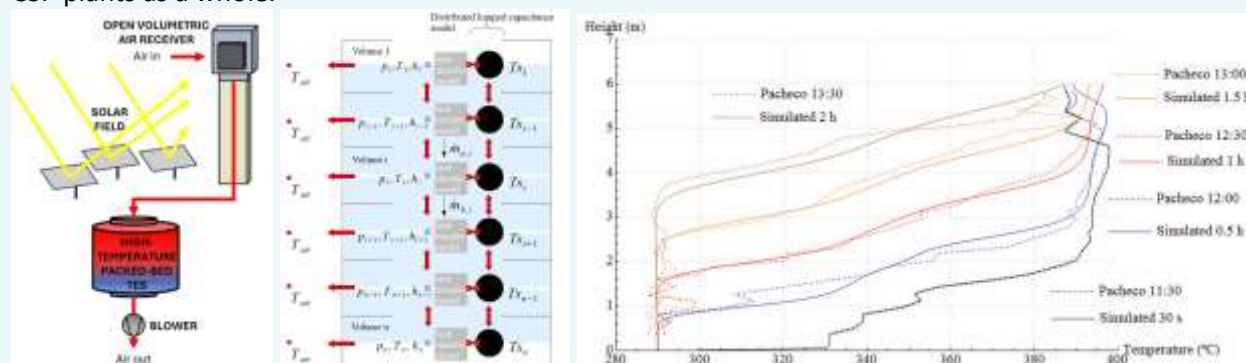
Figure 2: Thermocline TES concept (left); Thermocline TES model (center); Thermocline TES model validation (right)
