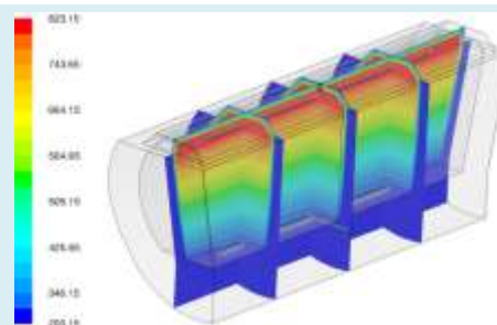
TES unit temperature contours (Temperature [K])
