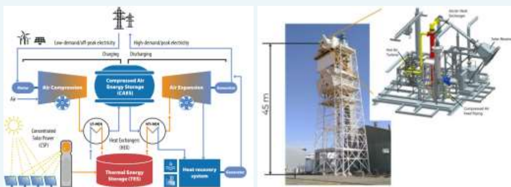
Figure 1: ASTERIx-CAESar concept (left); ASTERIx-CAESar main prototype at CIEMAT-PSA (right)
