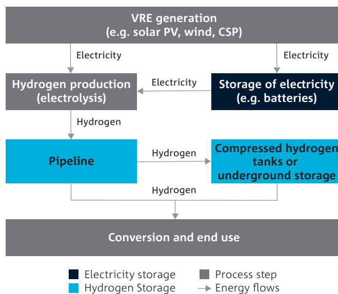
Figure 9: Storage options in hydrogen production
