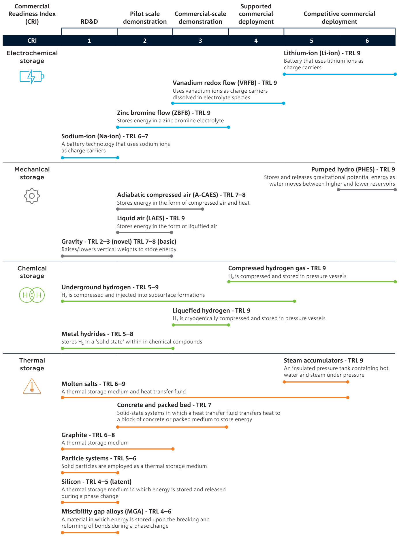
Figure 14: Summary of energy storage technology maturity
