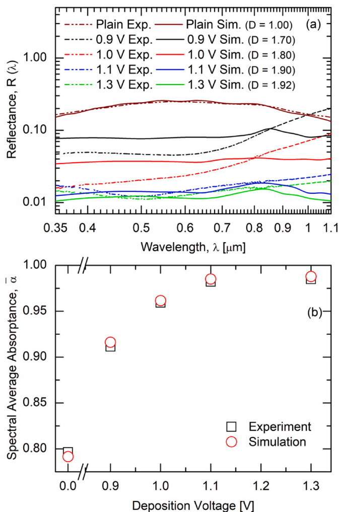
Fig. 10. Comparison of experimental and simulation: (a) spectral variation of reflectance (b) spectral average absorptance.
