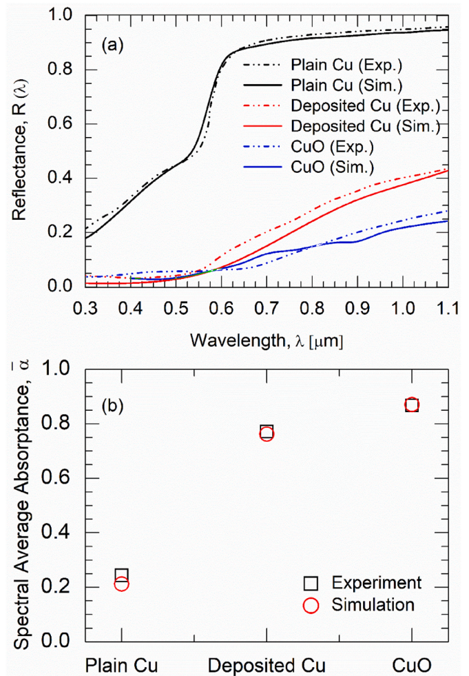
Fig. 9. Comparison of experimental and simulation results: (a) spectral variation of reflectance and (b) spectral average absorptance.
