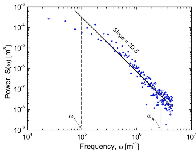
Fig. 2. Fast Fourier transform (FFT) based power spectrum of the surface in Fig. 1, showing the fractal characteristics of the surface over a frequency range.
