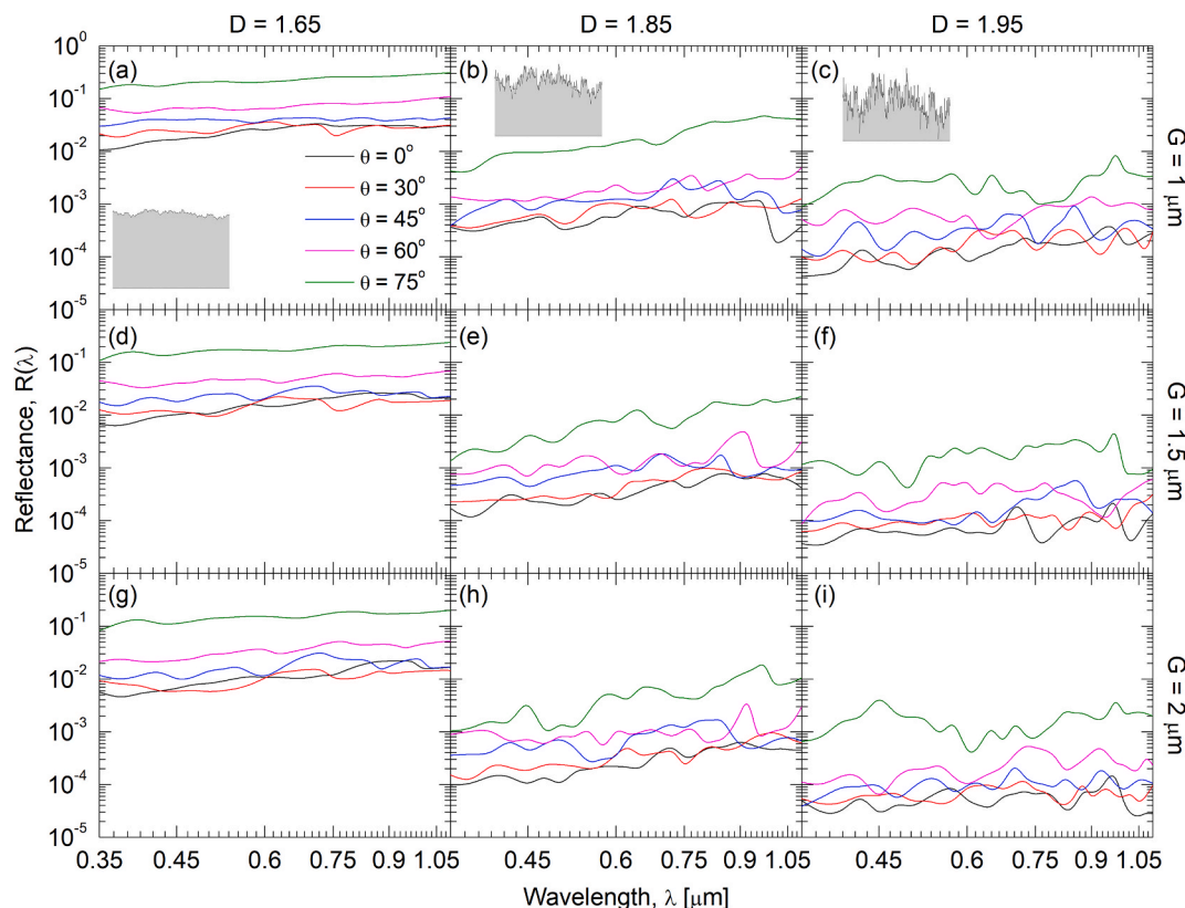
Fig. 4. Spectral variation of reflectance of CuMnO coatings at different incidence angles, for various combinations of fractal dimension, D , and scaling constant, G .
