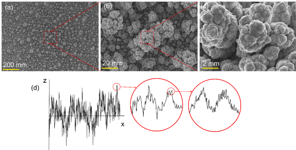
Fig. 1. (a–c) SEM images of an electrodeposited coating surface at different magnifications, (d) a representative profilometric line scan of the surface revealing self-affine characteristic of smaller length scale asperities being uncovered upon repeated higher magnification.
