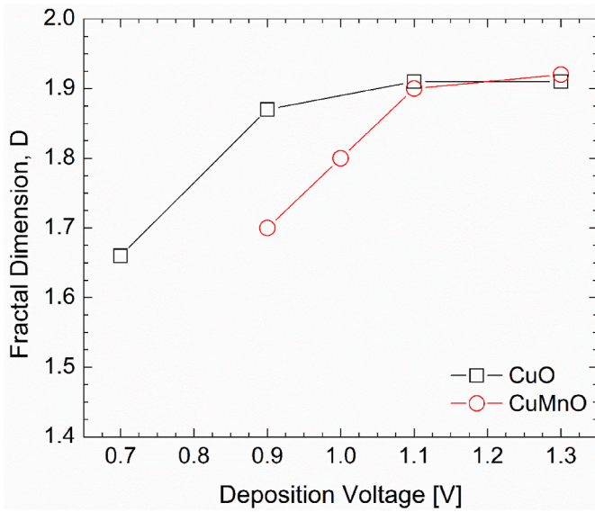
Fig. 8. Variation of the fractal dimension of CuO and CuMnO surfaces electrodeposited at various voltages.
