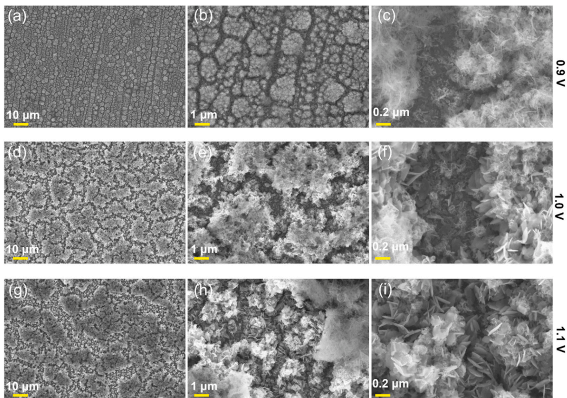
Fig. 7. SEM images at three different magnifications showing the morphologies of electrodeposited CuMnO coatings fabricated at (a,b,c) 0.9 V, (d,e,f) 1.0 V and (g,h,i) 1.1 V.
