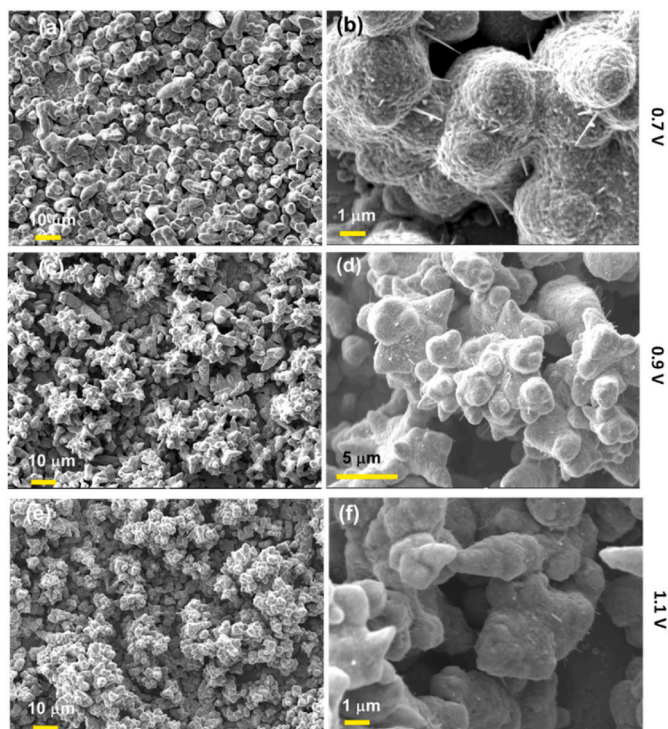
Fig. 6. SEM images at two different magnifications showing the morphologies of electrodeposited CuO coatings fabricated at (a,b) 0.7 V, (c,d) 0.9 V and (e,f) 1.1 V.
