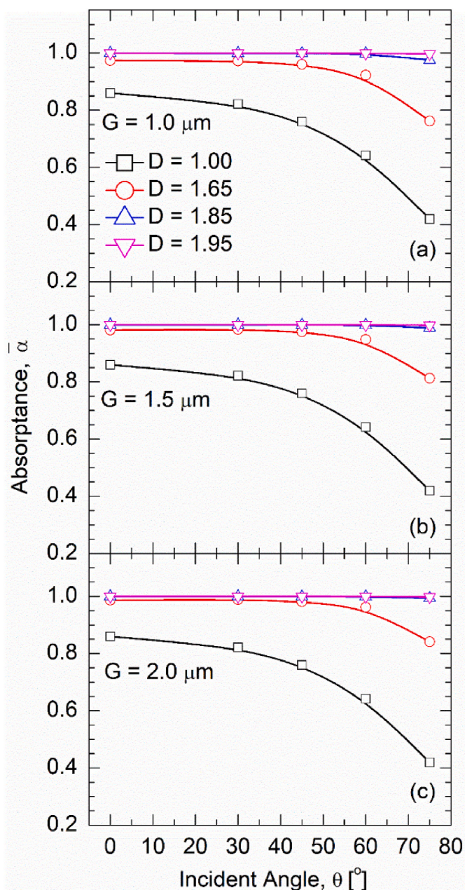
Fig. 5. Variation of spectrally averaged absorptance with incidence angle for different combinations of fractal dimension, D , and scaling constant, G .
