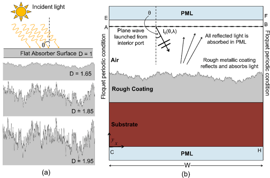
Fig. 3. Description of the optical model: (a) illustration of texture absorber surfaces based on the W-M function at different fractal dimensions; (b) schematic of the computational domain.
