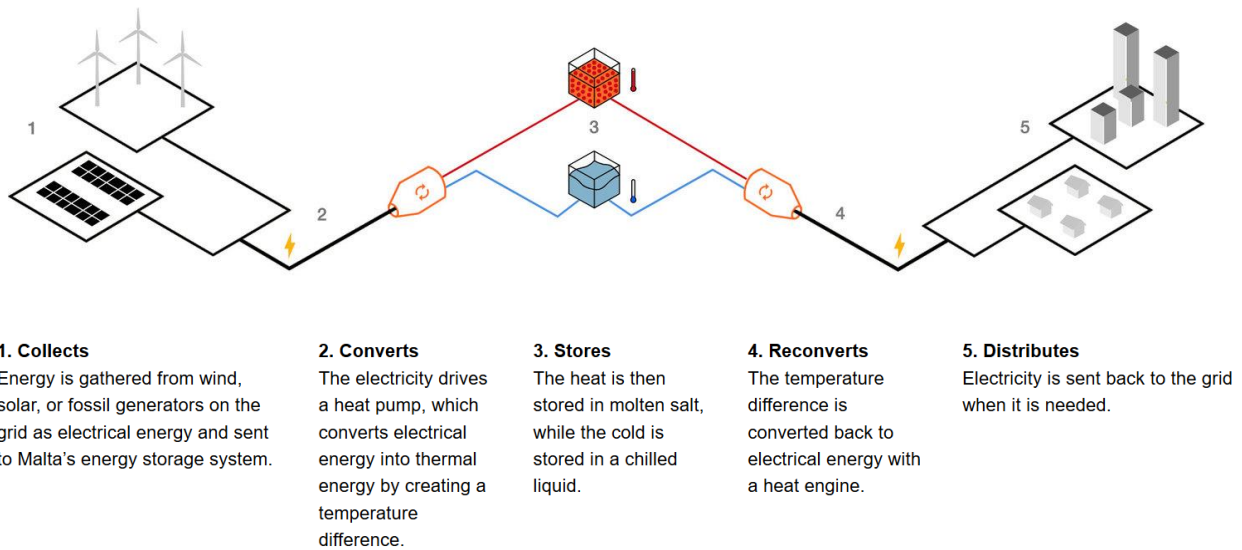
Figure 6. Malta's pumped thermal energy storage concept {Malta, 2020 #13799}
